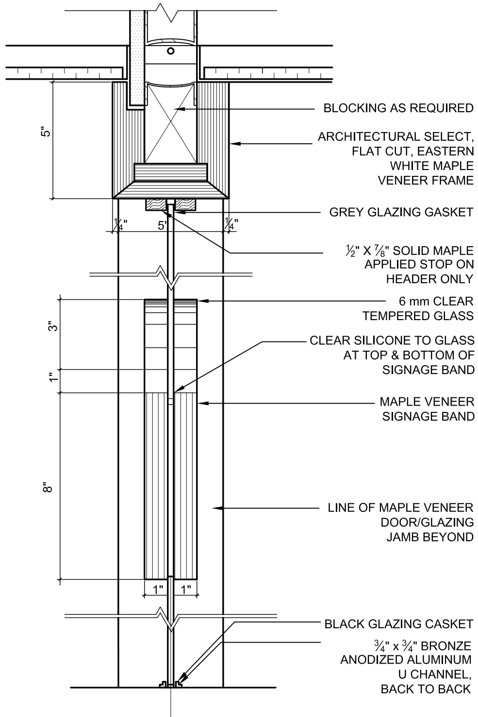
C TG-6 SECT. THRU GLAZING & MAPLE BAND & HEADER SCALE: 3" = 1'-0"
